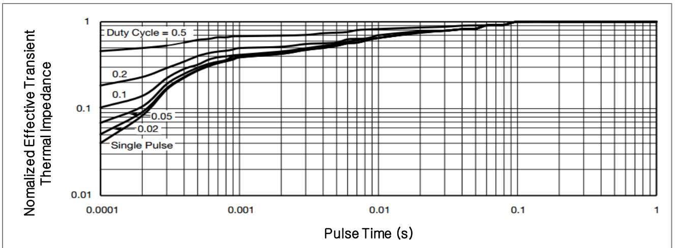
Fig 9 . Transient thermal impedance
